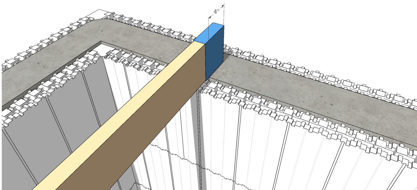
Figure 7 – Wood joist minimum bearing dimension
