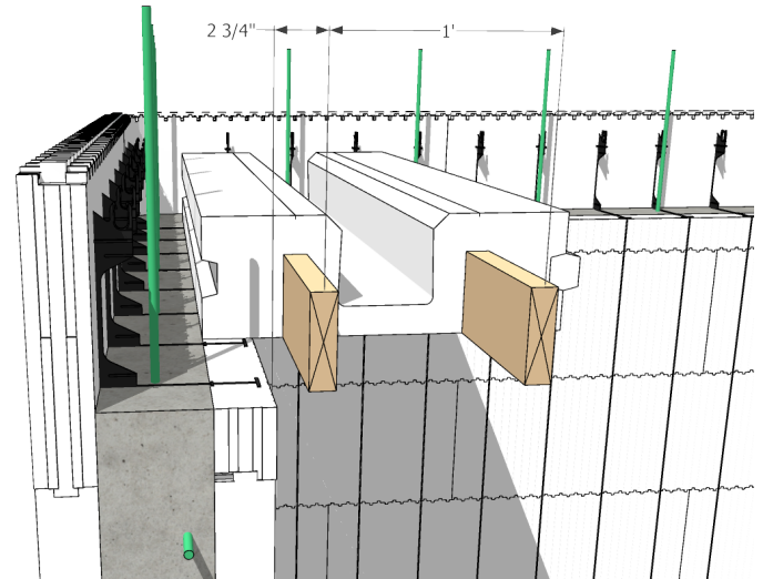
Figure 9 – First and second joist installation with R30 Amvic™ ICF
