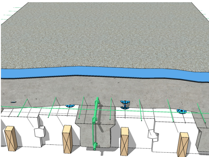
Figure 29 – Carpet with foam underpad
