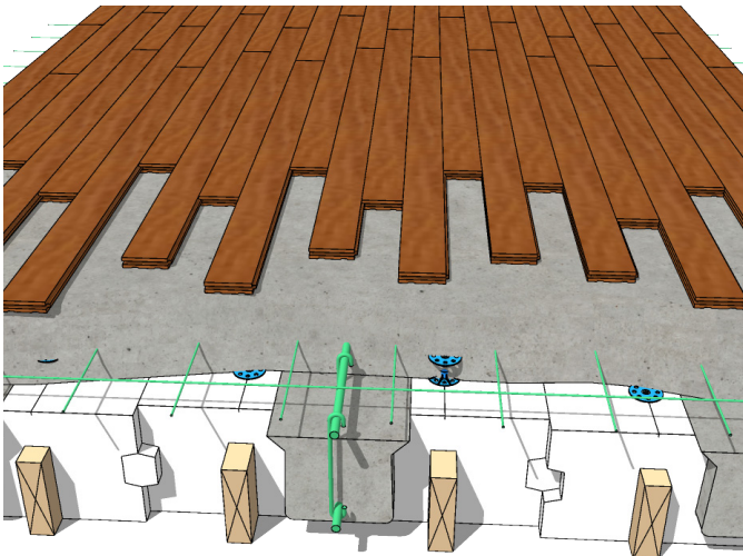
Figure 25 – Solid hardwood fully adhered to concrete
